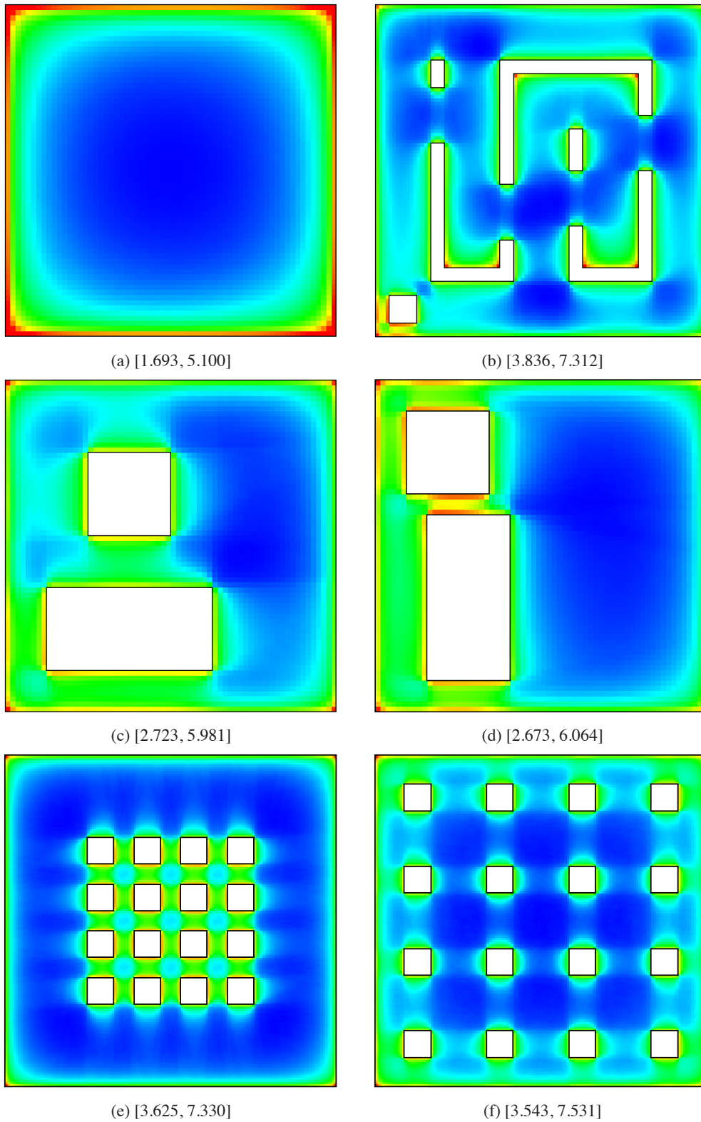
Figure 4: Complexity colour map and range of the complexity of a region for six scenes. Different grids have been used with 10^3 lines cast from each grid cell center.
