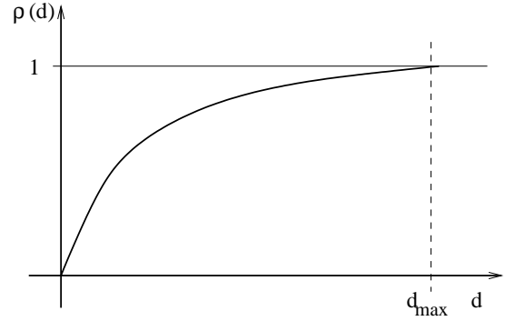
Figure 1: Shape of \rho(d) function.
