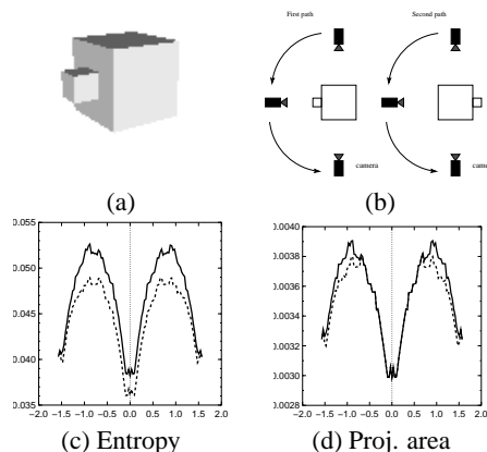
Figure 5: (b) depicts the paths of the camera around a pair of cubes. (c) and (d) show the entropy and projected area in the Y axis respectively against the rotation angle. The dashed line corresponds to the second path and the continuous one to the first.
